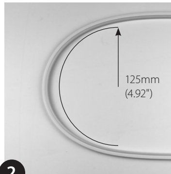
2 Recommended maximum bending radius is 125mm (4.92"). Over-bending can cause malfunction.
